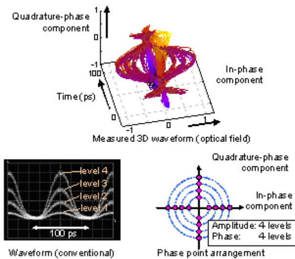
Fig. 3 Observation of 40 Gbps 16-level optical signal
