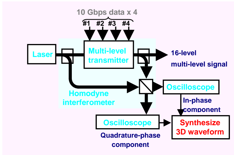
Fig.1 Set-up of 3D waveform (optical field) measurement
