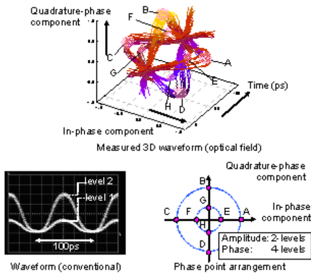
Fig. 2 Observation of 30 Gbps 8-level optical signal
