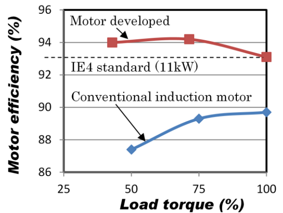
Fig. 4. Comparison of motor efficiency (11kW)
